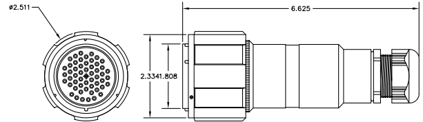
TL-54-LF06: 54 PIN FEMALE CABLE MOUNT CONNECTOR
