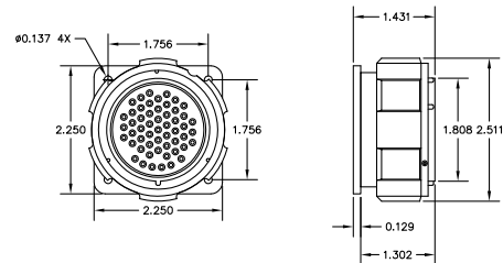
TL-54-PF26: 54 PIN FEMALE PANEL MOUNT CONNECTOR
