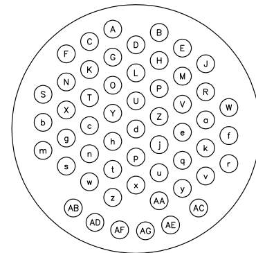
TL-54-PF26: 54 PIN FEMALE CONNECTOR
