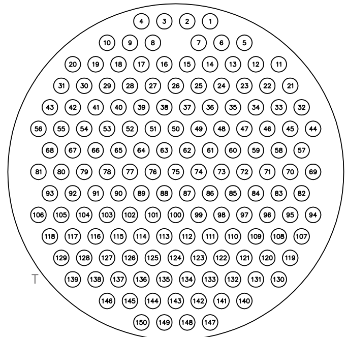
TL-150-PM02: 150 PIN MALE CONNECTOR
