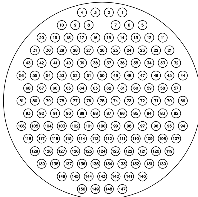
TL-150-PM02: 150 PIN MALE CONNECTOR
