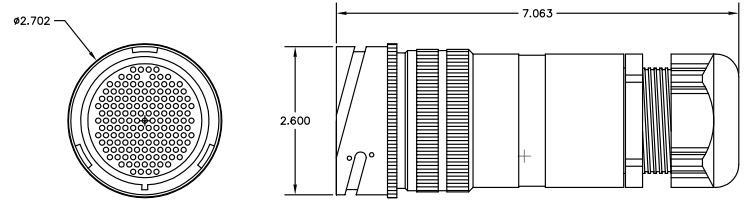
TL-150-LM01: 150 PIN MALE CABLE MOUNT CONNECTOR
