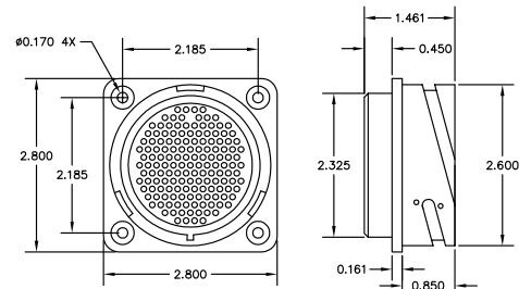
TL-150-PM02: 150 PIN MALE PANEL MOUNT CONNECTOR
